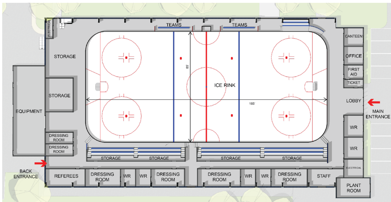
PLAN – EXISTING – FIRST FLOOR
