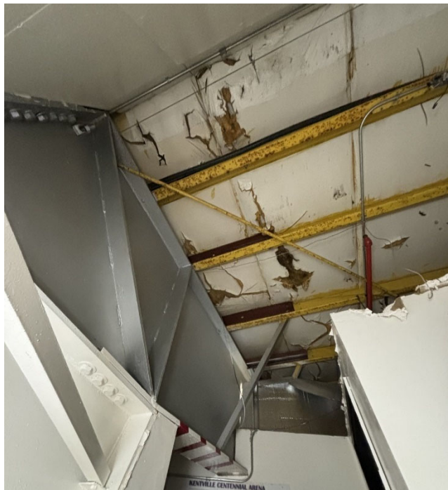
View of roof purlins and underside of roof assembly
