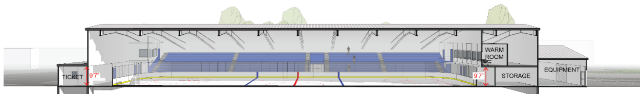
SECTION 2 – EXISTING
