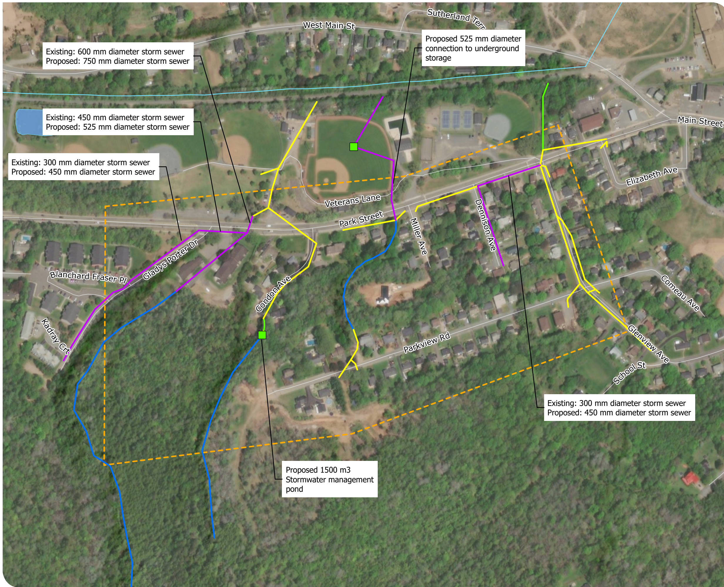
PROPOSED UPGRADES AREA OF CONCERN 3 : RESIDENTIAL AREA SOUTH OF PARK STREET FIGURE #7-3
