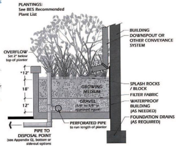
Figure 7-11: Conceptual Sketch of Bioretention Cell Components (TRCA, nd)
